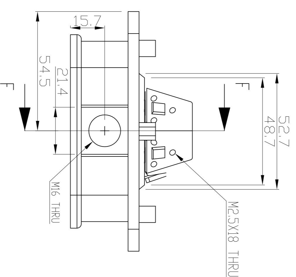
SIDE VIEW
